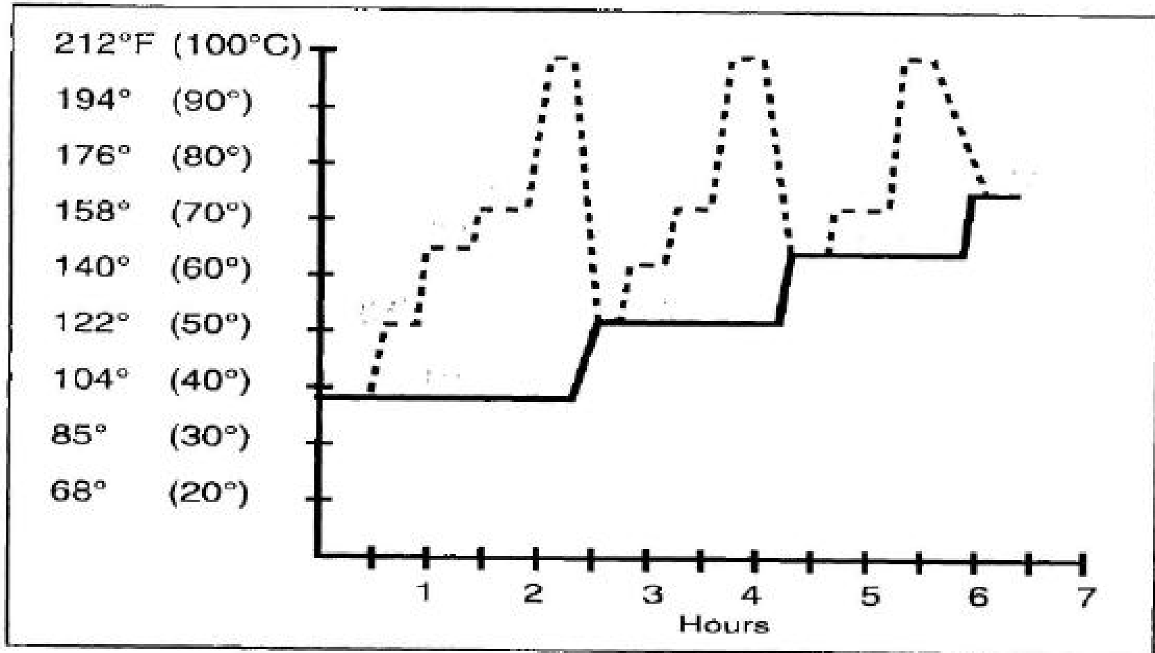
Mash program at Bavarian State Brewery at Weihen – Stephan: Typical three-decoction mash program.
